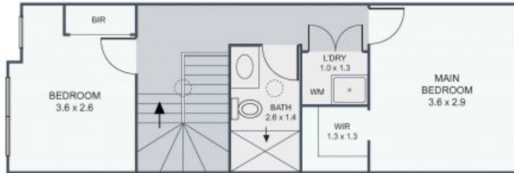
FIRST FLOOR
