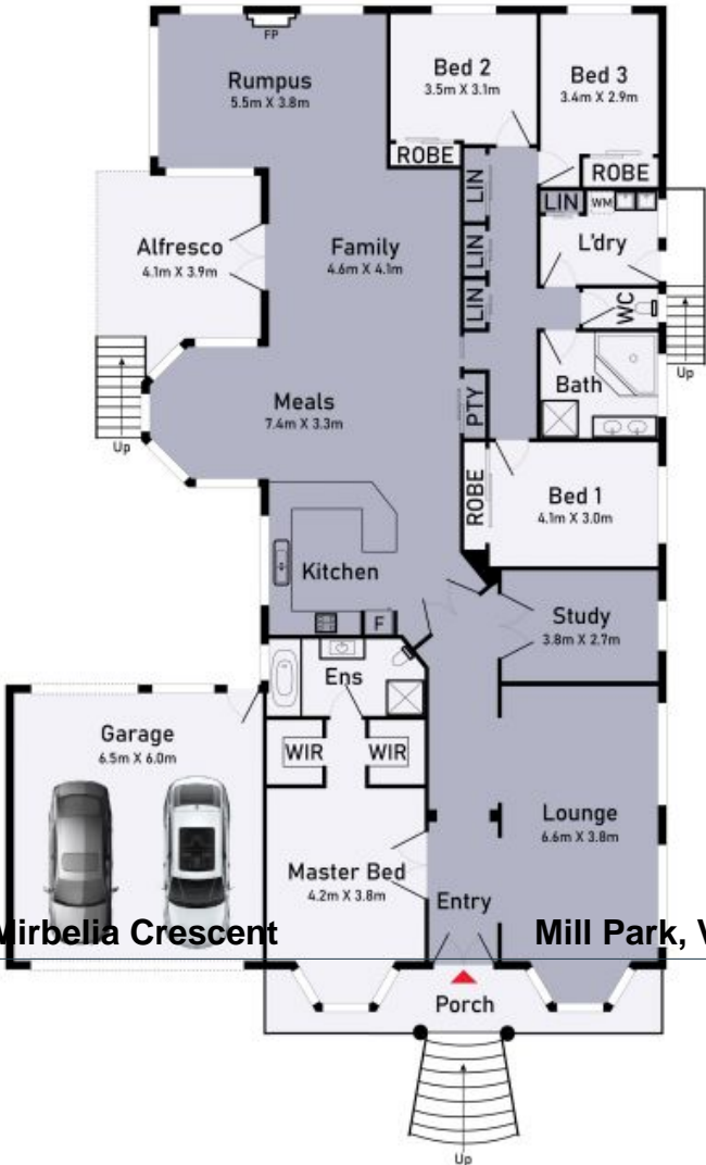
Floor Plan
