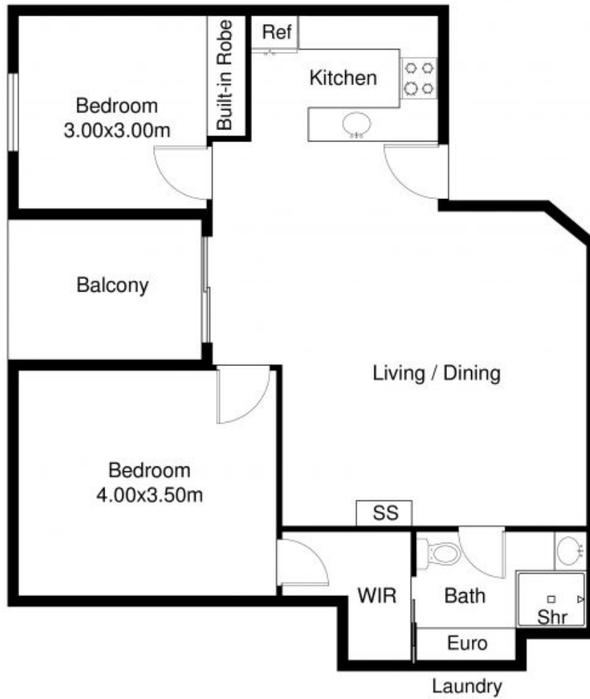
FLOOR PLAN
