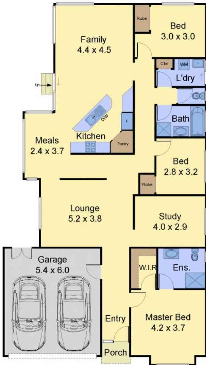
FLOOR PLAN
