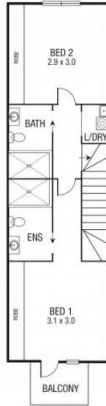
SECOND FLOOR
